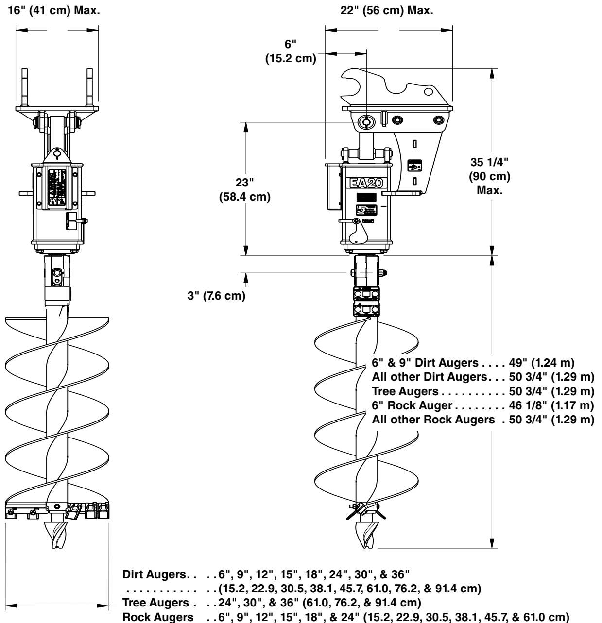
Dirt auger shown with mount #317-247A
