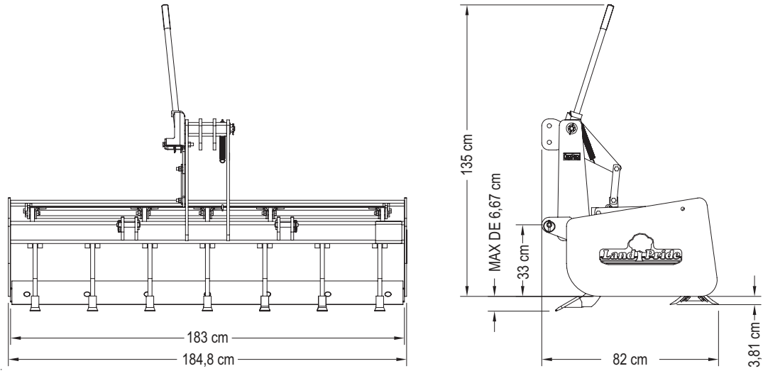
Lame niveleuse escamotable MR1572
