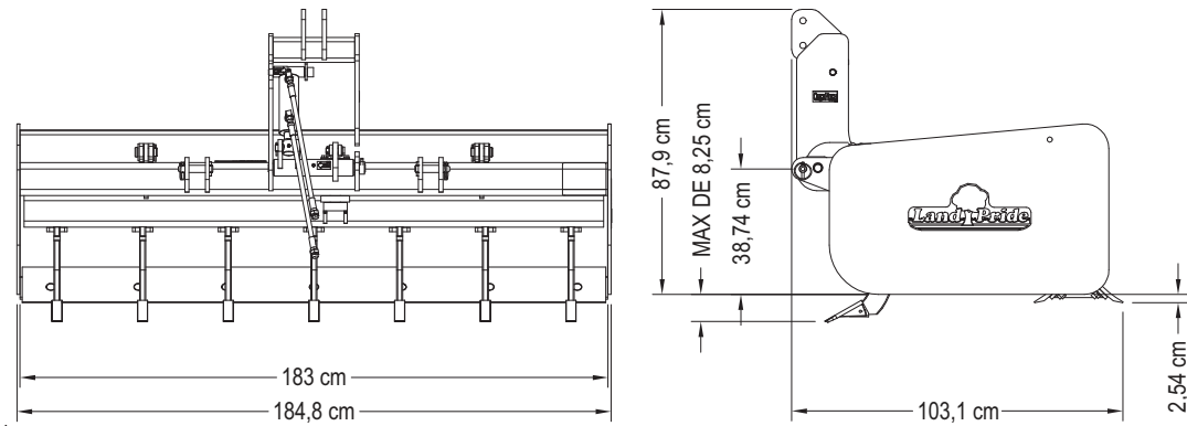
Lame niveleuse escamotable HR2572
