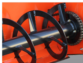
Augers are 3/8" x 2-1/2" with 14" or 16" diameter, and are protected by a shear-bolt.
